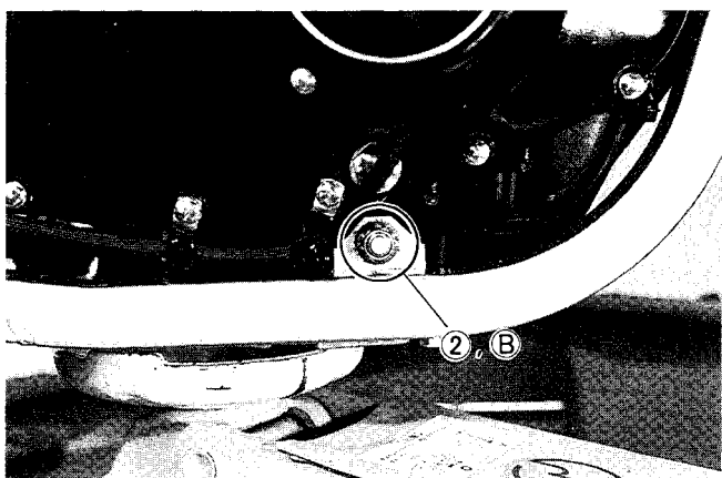
② BOLT LENGTH : 240 mm (9.45 in) Ⓑ SPACER LENGTH : 16.8 mm (0.66 in) ... 2 pcs.
