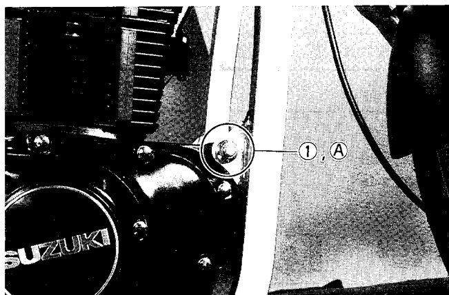
① BOLT LENGTH : 255 mm (10.04 in) Ⓐ SPACER LENGTH : 65 mm (2.56 in) ... 2 pcs.
